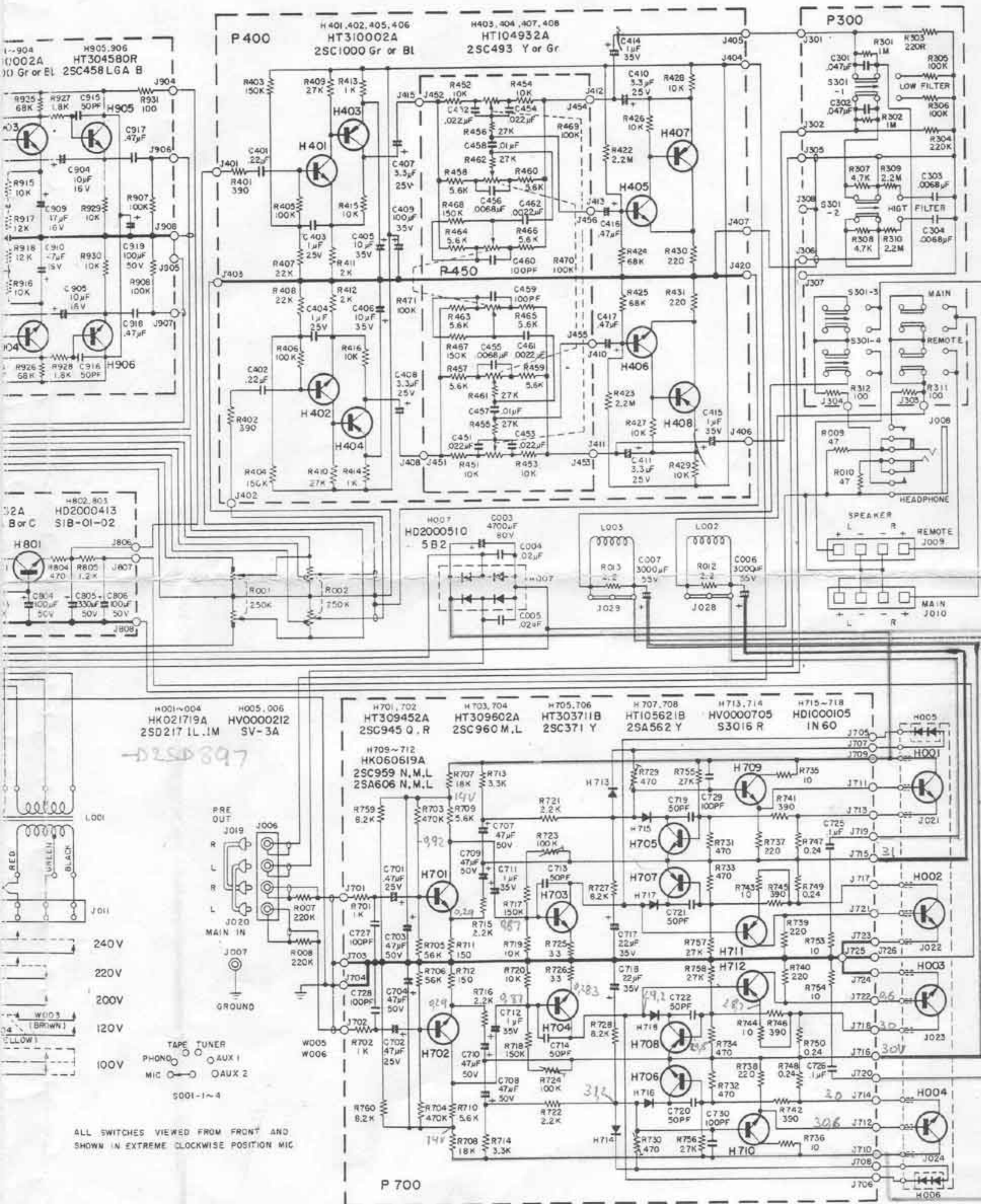
Figure 16. Schematic Diagram
